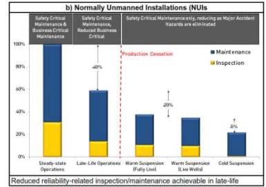
Figure 1 Reduced Inspection/Maintenance of Production/Safety-critical Elements after Production Ceases & Accident Hazards are eliminated.
